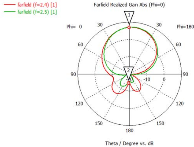
Elevation Pattern
