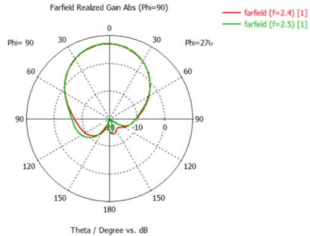
Horizontal Pattern
